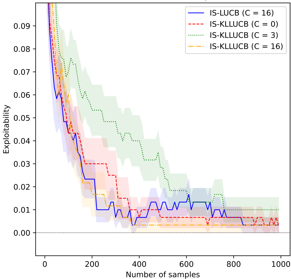
Kuhn Poker, KLUCB, Player o
